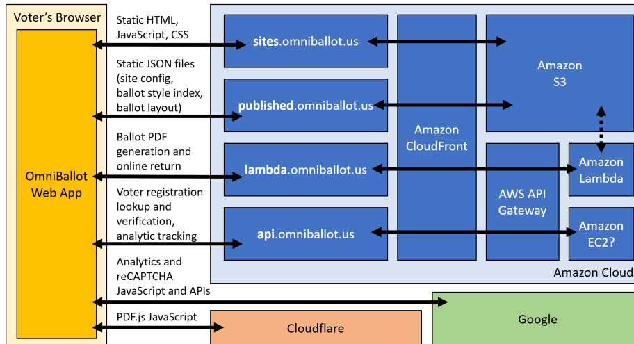
Fig. 2: OmniBallot architecture. The web app runs in the browser and uses HTTPS to load files and call REST-like APIs from several domains. When voting online or marking a ballot, the app sends the voter’s identity and ballot selections to Democracy Live services running in Amazon’s cloud. The app runs JavaScript loaded from Amazon, Google, and Cloudflare, making all three companies (as well as Democracy Live itself) potential points of compromise for the election.
